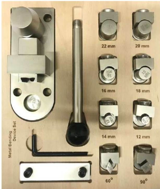
VI - 240 Ring Bending Device With Wooden Base
