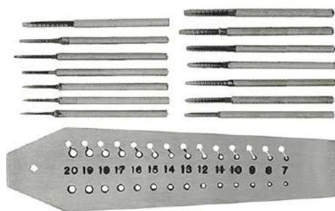
VI - 88 Screw Plate With 14 Taps (0.7 mm To 2 mm)
