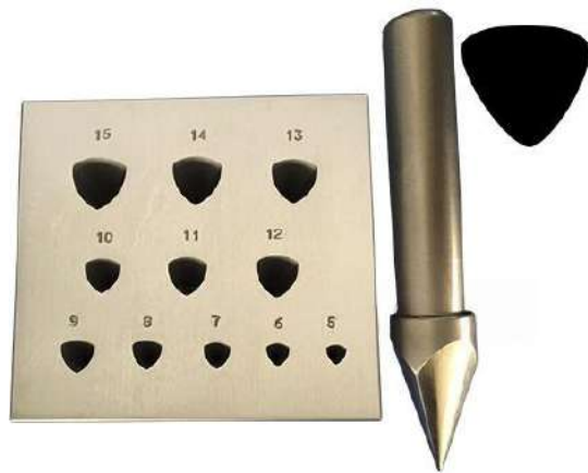
VI -500 Bezel Block Trillion Shape Hole with 17 Degree Punch
